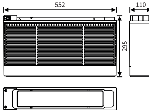
Dimensions (mm)
