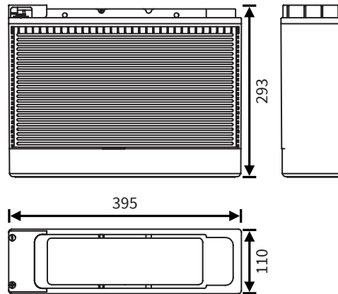
Dimensions (mm)
