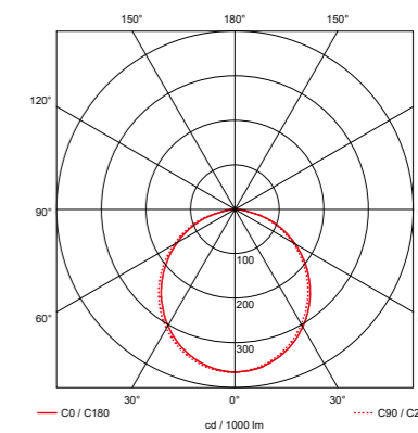
Downlight IP44
