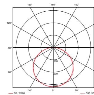
Rockdisc III
